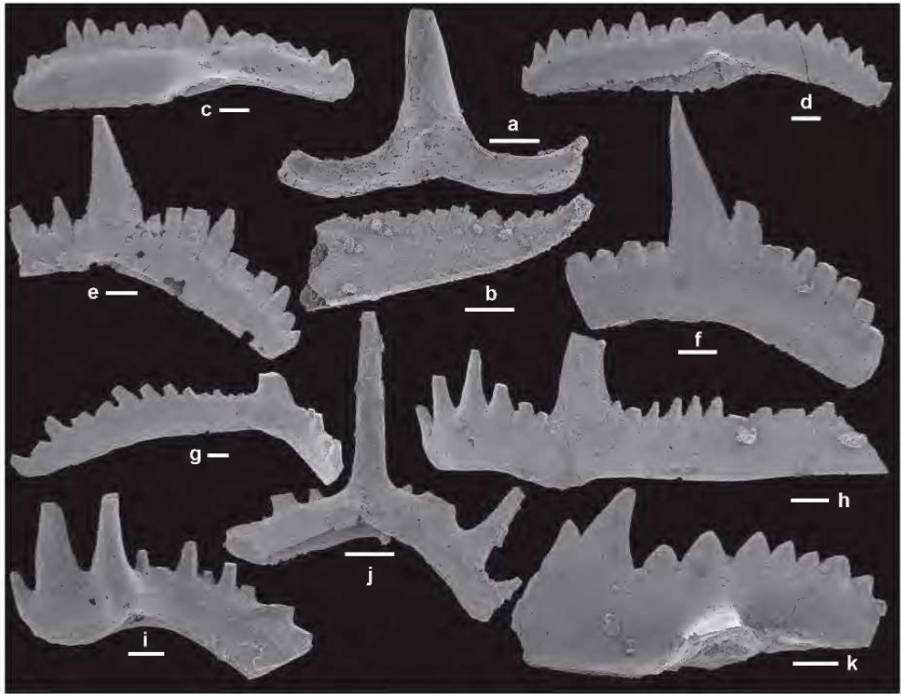
Fig. 6. a, Oulodus astriatus ? Mathieson, Mawson, Simpson and Talent, 2016. Sa element, MMMC5231, from sample C2817 (Louth L2), posterior view (IY310-001). b, Belodella resima (Phillip, 1965). Sc element, MMMC5232, from sample C0816 (DDH K1), inner-lateral view (IY308-006). c-h, Wurmiella excavata (Branson and Mehl, 1933). c-d, Pa element; c, MMMC5233, from sample C0987 (DDH K6), inner-lateral view (IY310-004); d, MMMC5234, from sample C0987 (DDH K6), outer-lateral view (IY310-005); e-f, Pb element; e, MMMC5235, from sample C0987 (DDH K6), inner-lateral view (IY310-002); f, MMMC5236, from sample C0987 (DDH K6), outer-lateral view (IY310-003); g-h, Sc element; g, MMMC5237, from sample C0987 (DDH K6), inner-lateral view (IY310-006); h, MMMC5238, from sample C0987 (DDH K6), posterior view (IY310-007). i-j, Oulodus spicula Mawson, 1986. i, Sb element, MMMC5239, from sample C0987 (DDH K6), posterior view (IY310-008); j, Sa element, MMMC5240, from sample C0986 (DDH K6), posterior view (IY310-011). k, Pandorinellina exigua philipi (Klapper, 1969). Pa element, MMMC5241, from sample C0987 (DDH K6), outer-lateral view (IY310-009). Scale bar 100 \mu m.
